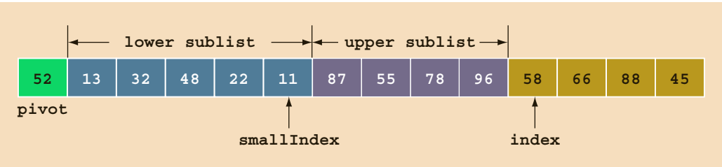
FIGURE 18-26 List before moving 58 into a sublist
