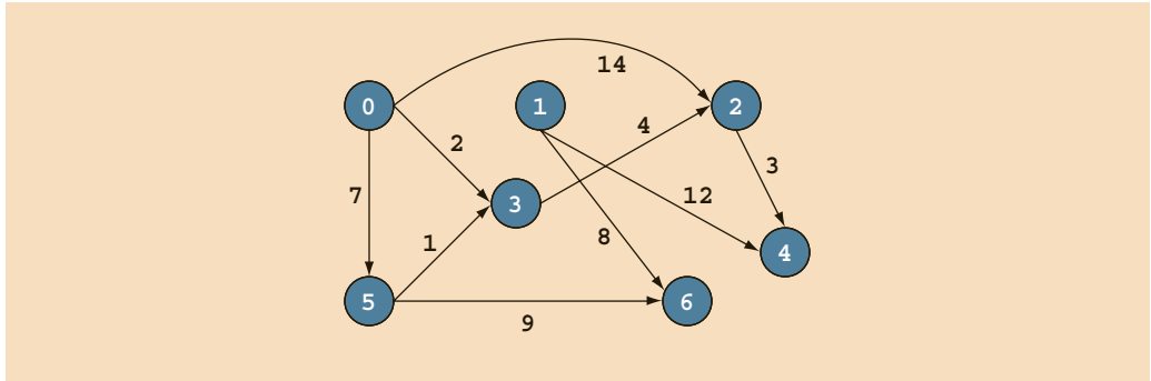
FIGURE 20-19 Graph for Exercise 17
