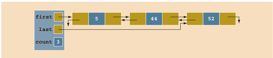
FIGURE 16-44 List after deleting the node with info 17
