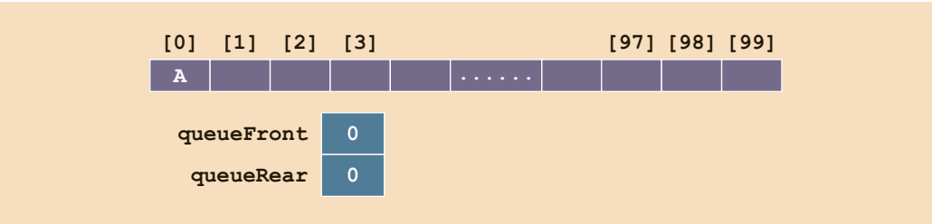
FIGURE 17-26 Queue after the first addQueue operation
