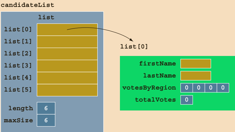
FIGURE 18-40 candidateList
