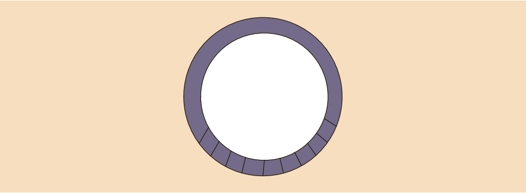
FIGURE 17-30 Circular queue
