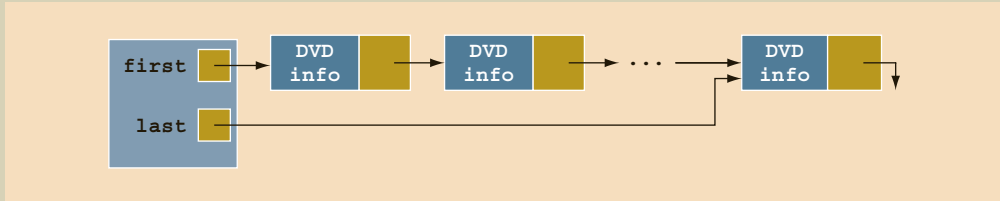
FIGURE 16-46 dvdList
